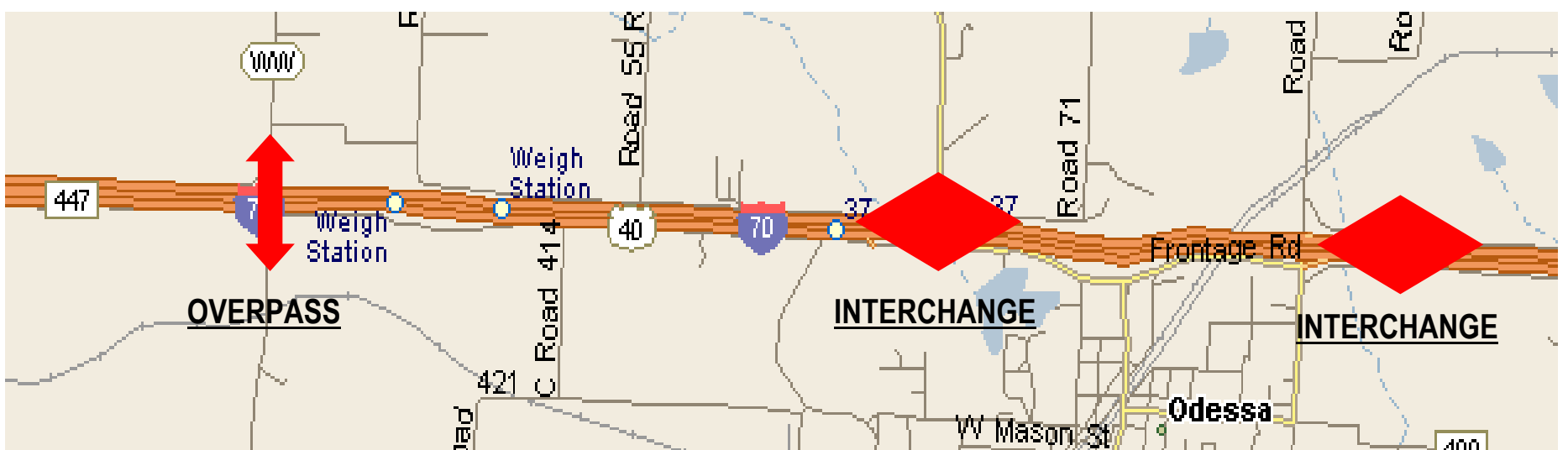
Option C- New interchanges at Route 131 and Johnson Road with an overpass at Route WW.
