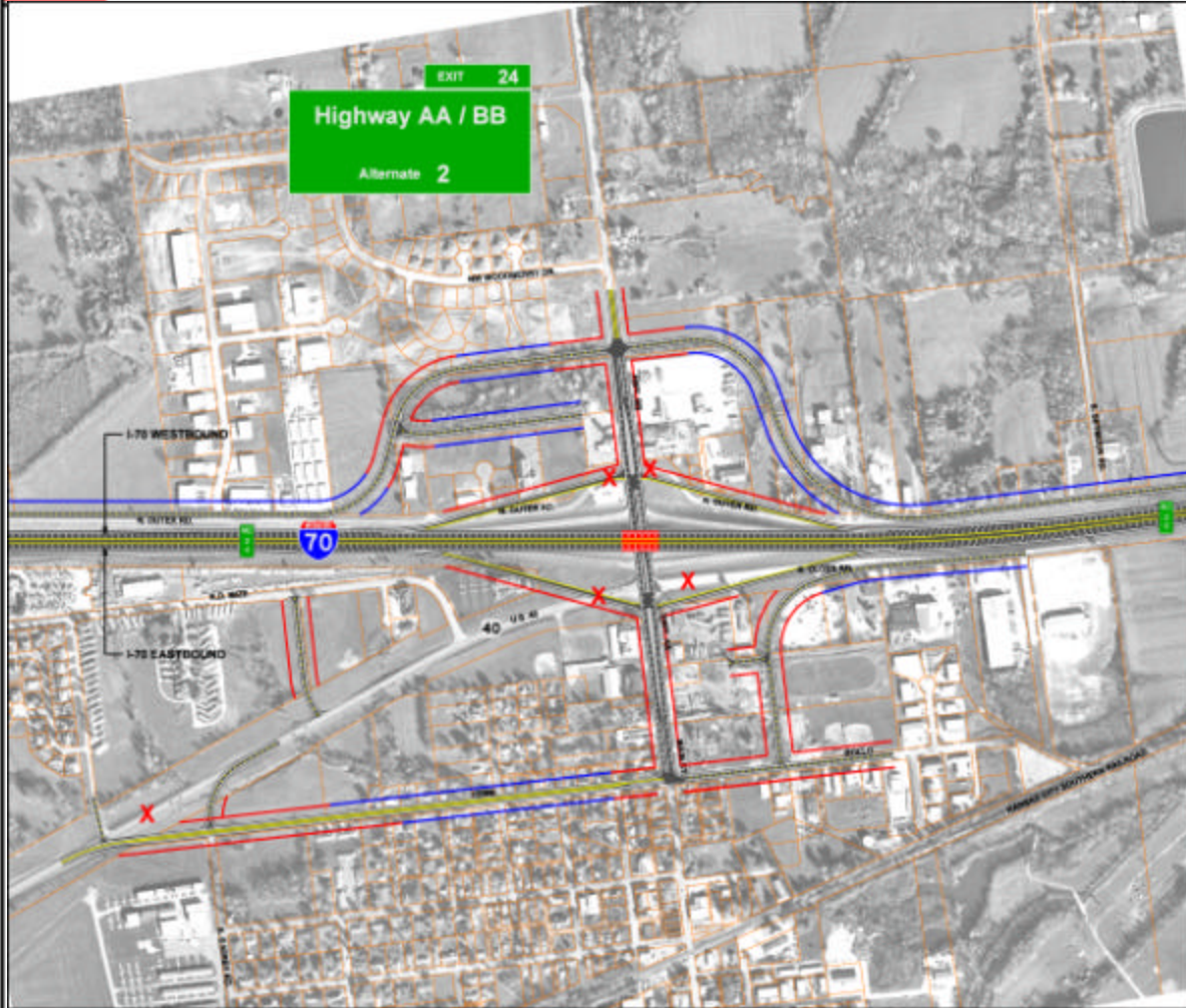
ALTERNATE 2 DIAMOND INTERCHANGE AT HIGHWAY AA / BB
