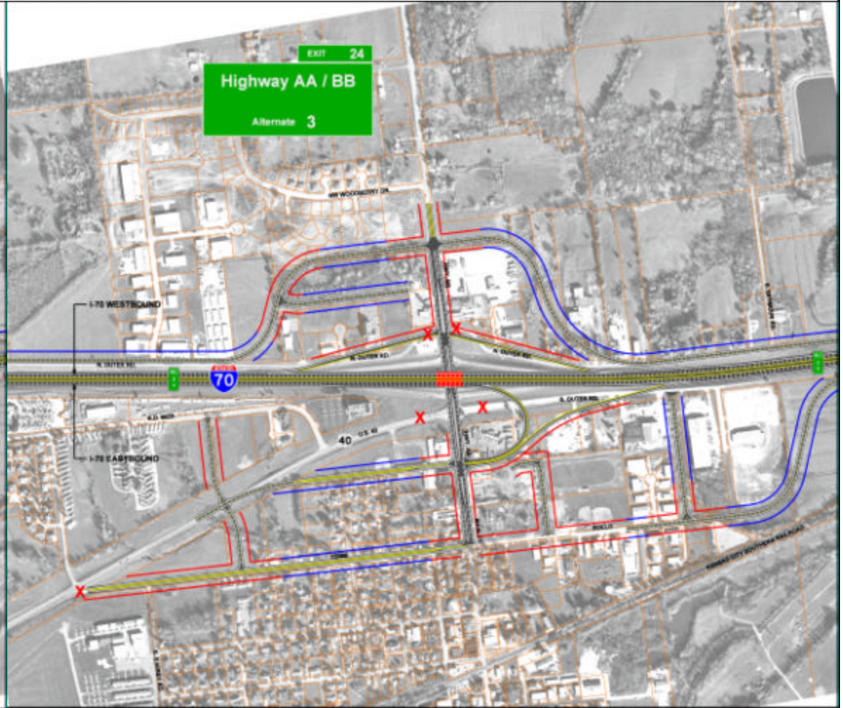
ALTERNATE 3 FOLDED DIAMOND INTERCHANGE AT HIGHWAY AA / BB
