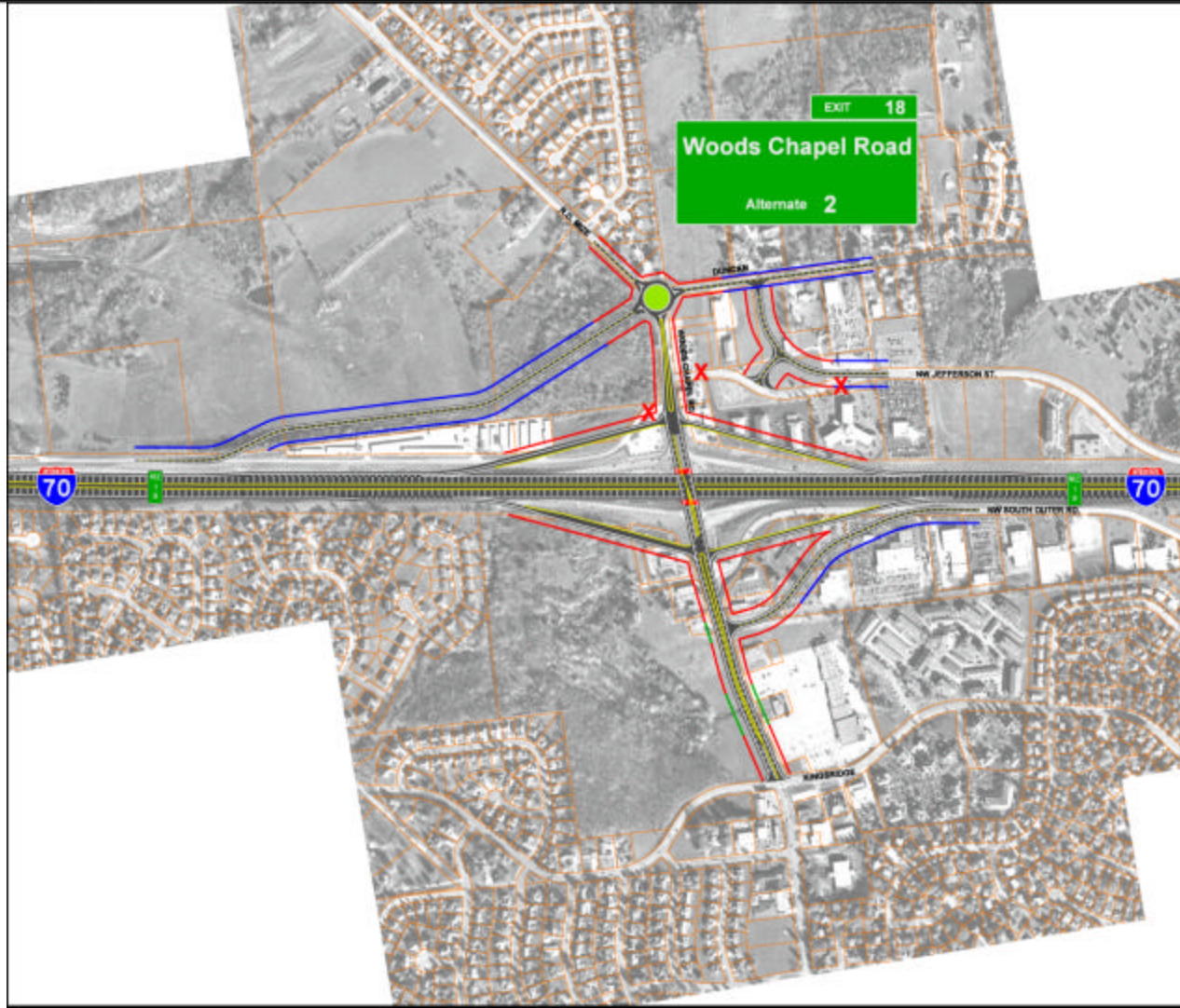
ALTERNATE 2 DIAMOND INTERCHANGE AT WOODS CHAPEL ROAD
