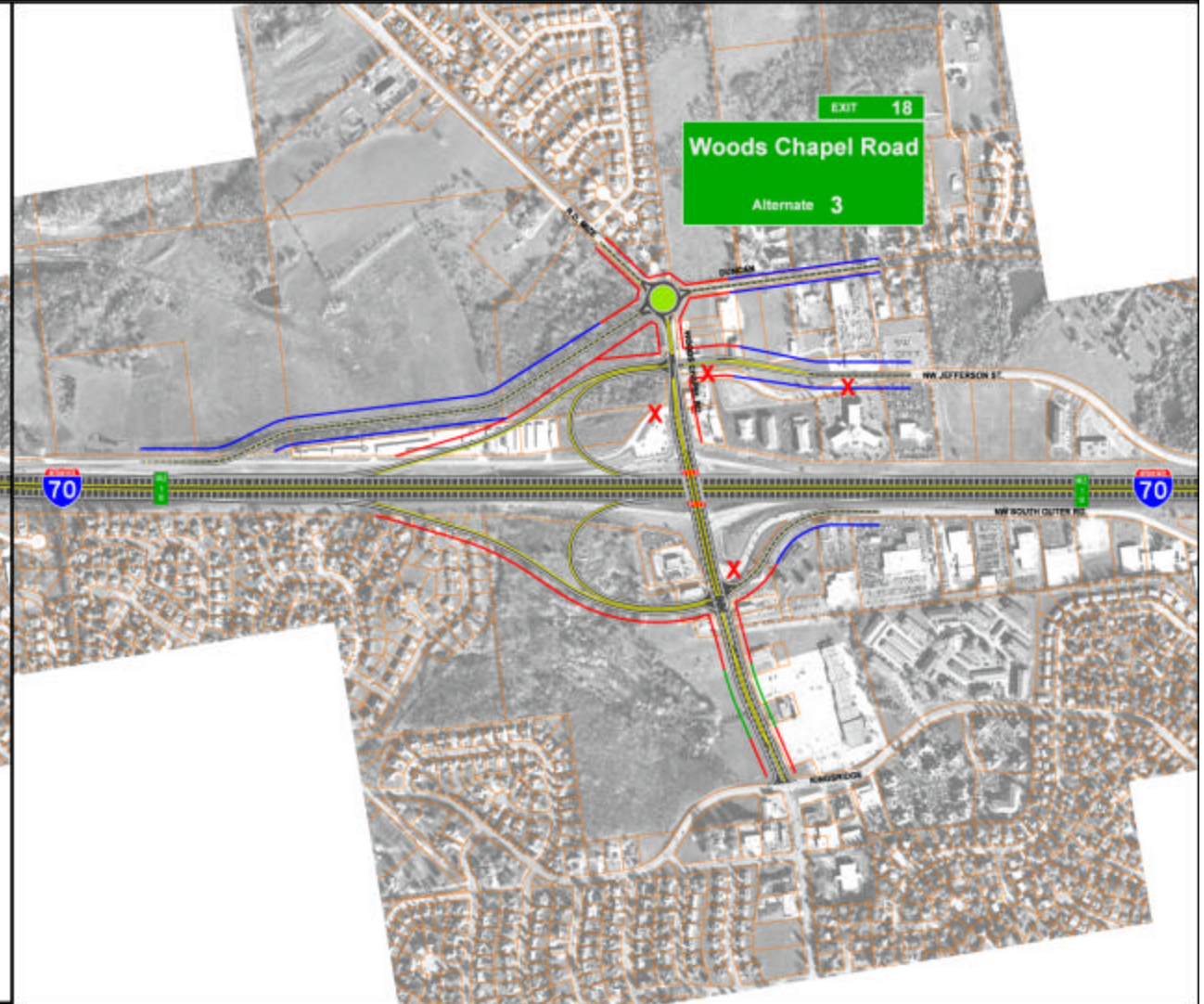
ALTERNATE 3 FOLDED DIAMOND INTERCHANGE AT WOODS CHAPEL ROAD
