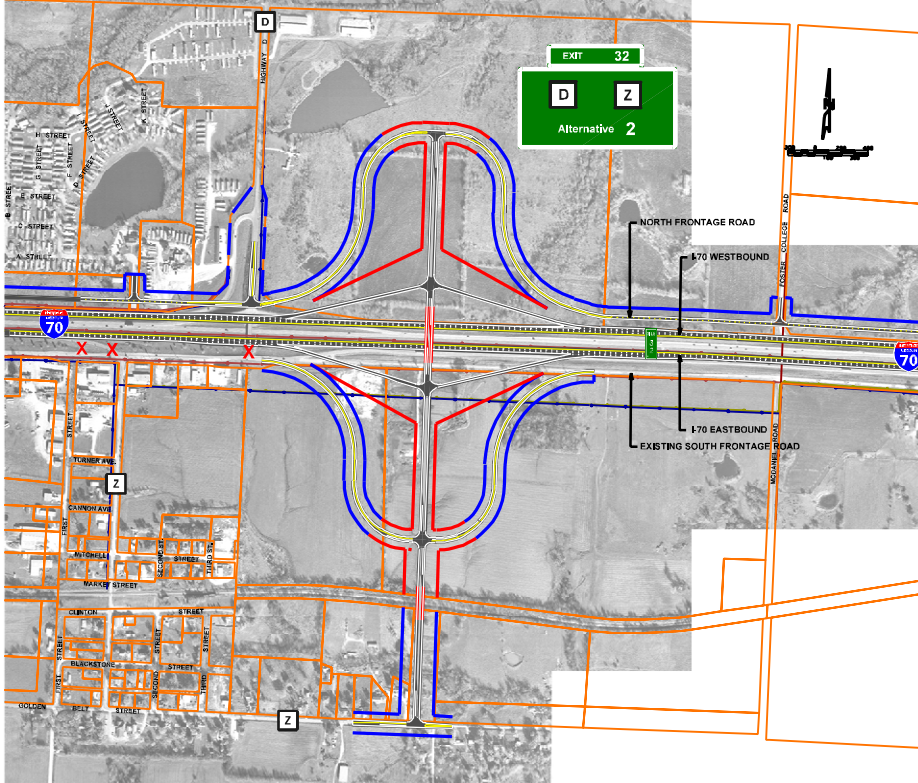
ALTERNATIVE 2 DIAMOND INTERCHANGE 1/4 MILE EAST OF HIGHWAY D
