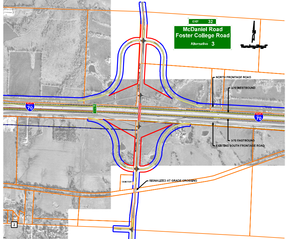
ALTERNATIVE 3 DIAMOND INTERCHANGE AT MCDANIEL ROAD/ROUTE Z
